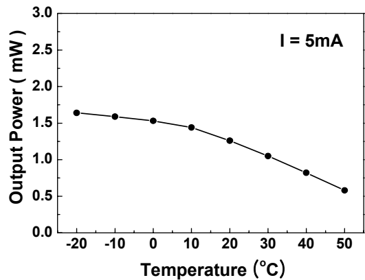
P_o vs Temperature
