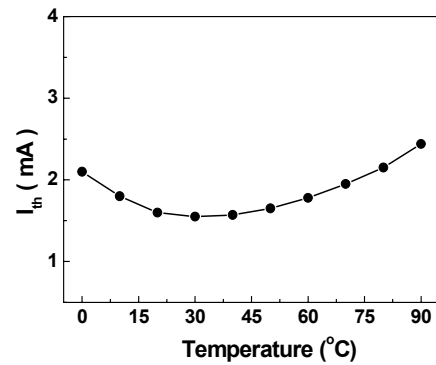
I th vs Temperature
