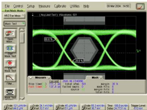
Eye diagram
