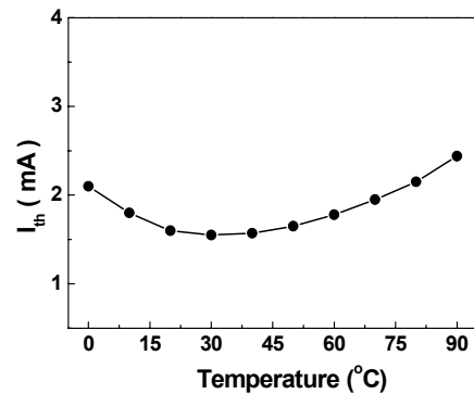
I th vs Temperature
